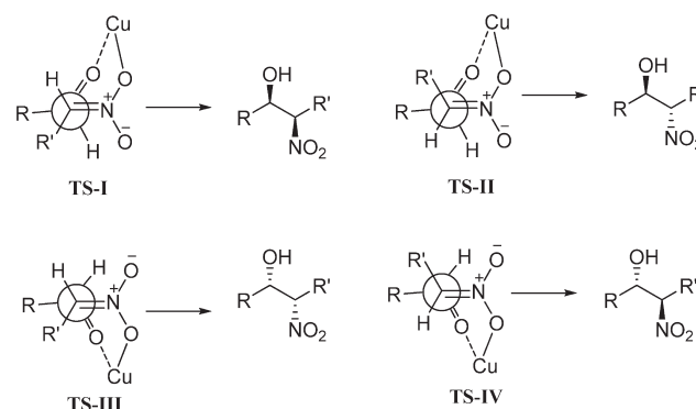
FIGURE 2. Plausible transition state for the diastereoselective Henry reaction.
